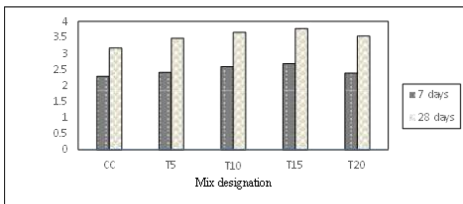
Figure 3 Variation of splitting tensile strength with different TPWFS contents at 7&amp;28 days.
